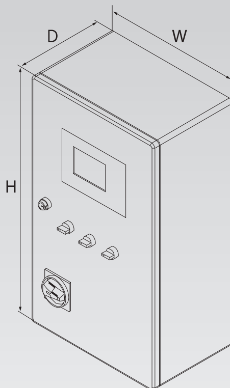
Figure 31: EHP Series Panel Dimensions
