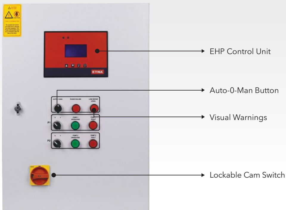
Figure 1: EHP Series Panel Exterior
