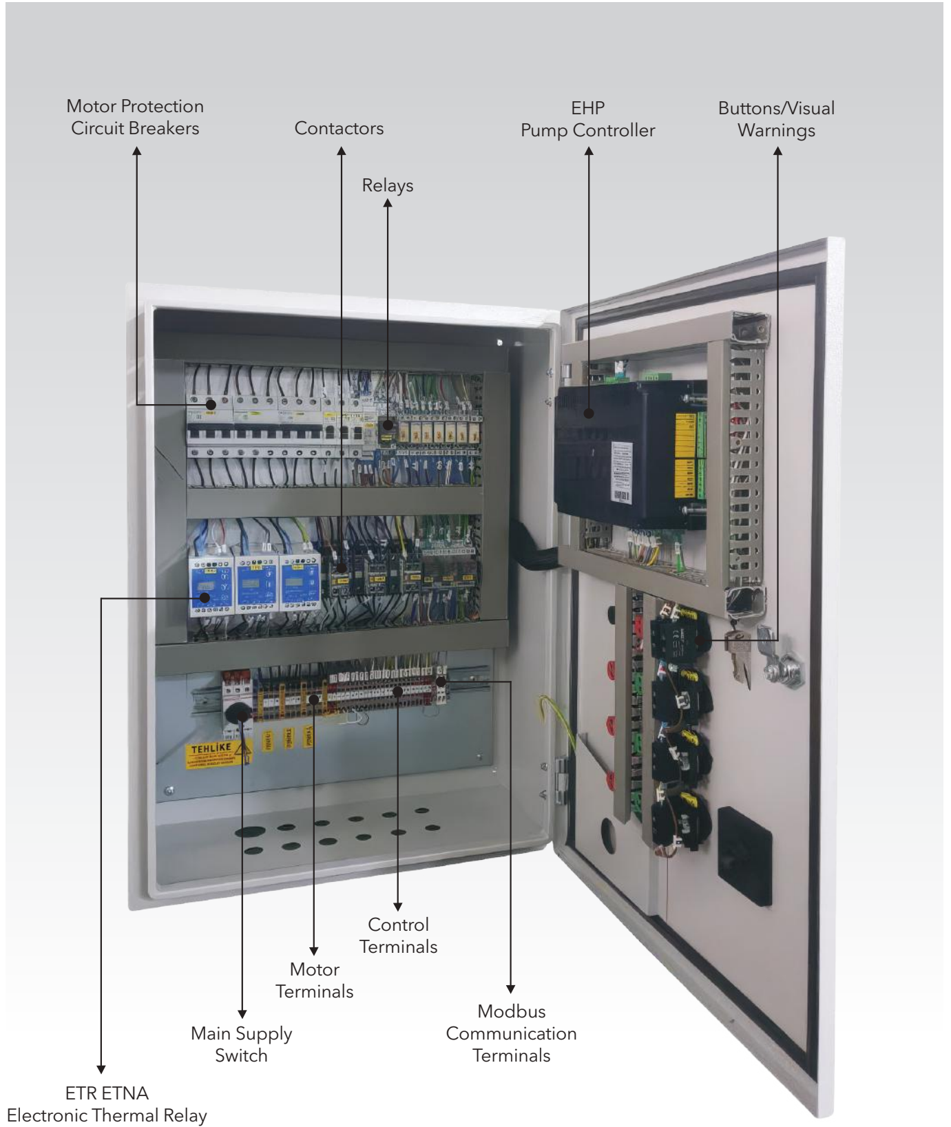
Figure 2: EHP Series Panel Interior
